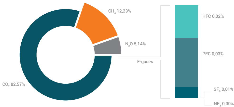
Fig. 1. Share of individual GHGs in the total domestic emissions 1988 (w/o LULUCF)
