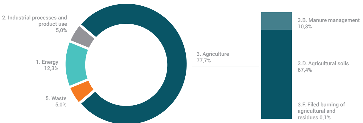
Fig. 30. Nitrous oxide emissions (w/o LULUCF) in 2016, by category
