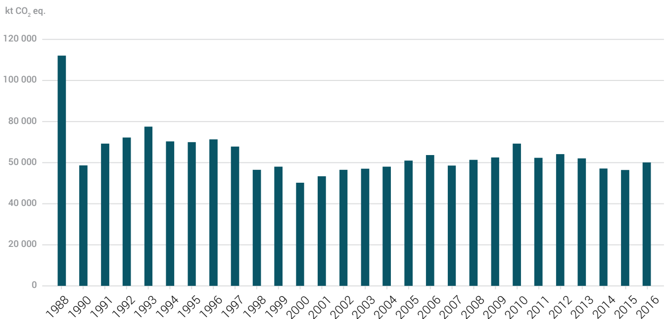
Fig. 27. Emission trend for the IPCC 1.A.4 sector. Other (covering service buildings and institutions, residential buildings and buildings used in agriculture, fishing and hunting) in 1988-2016. Including all greenhouse gases recalculated to CO 2 eq
