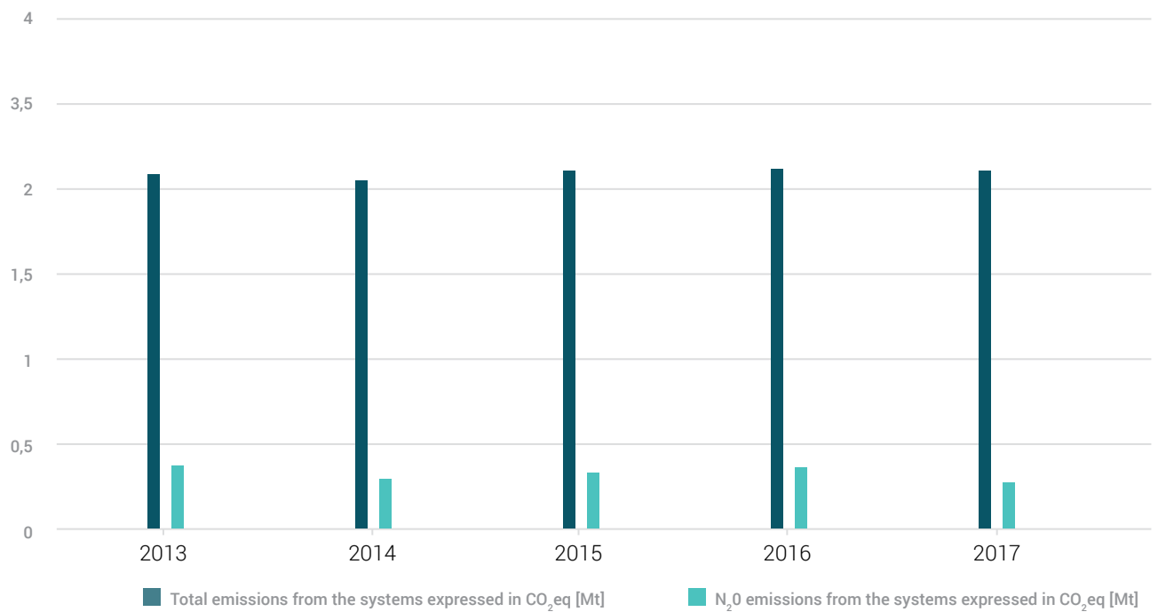
Fig. 36. Installations reporting nitrous oxide emissions, covered by EU ETS since, expressed in Mt CO 2 eq
