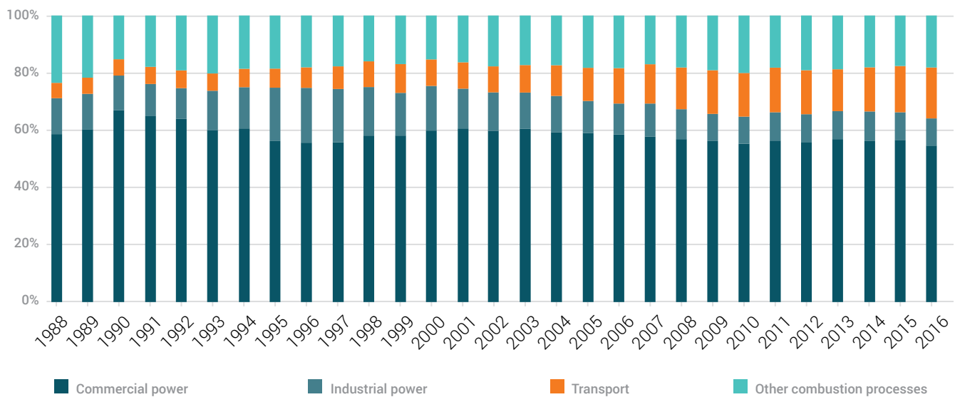
Fig. 11. Sectoral share in the fuel combustion emission balance, 1988-2016
