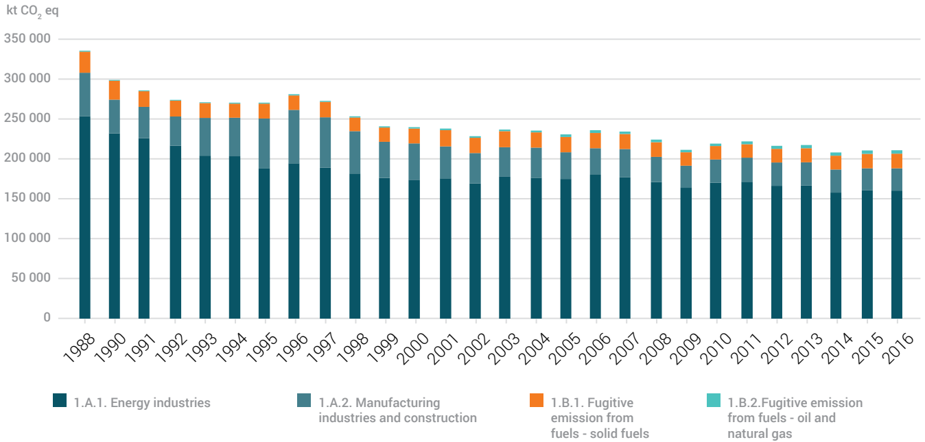
Fig. 14. Emission trend for the IPCC 1 sector. Energy in the years 1988-2016 divided into sub- sectors. Including all greenhouse gases recalculated to CO 2 eq without emissions from transport (1.A.3) and buildings (1.A.4)
