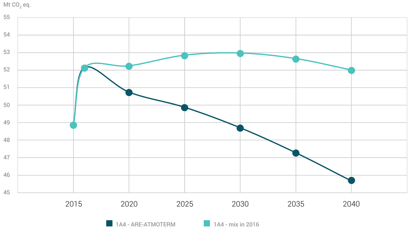
Fig. 64. Change in the greenhouse gas emissions resulting from the alteration of the fuel mix in the small combustion sources (sector 1.A.4.)
