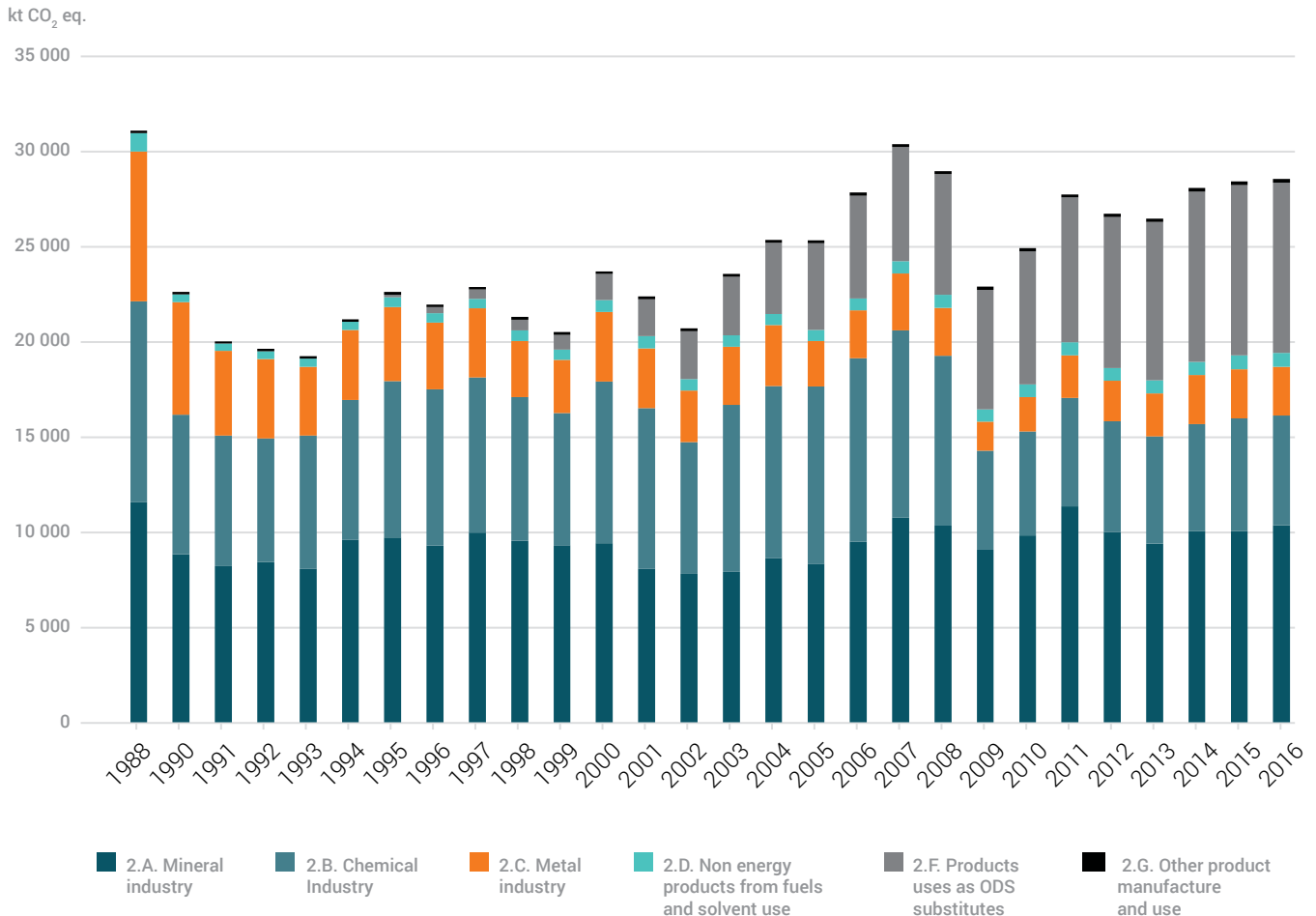
Fig. 19. Emission trend for the IPCC 2 sector. Industrial processes and product use in the years 1988-2016 divided into sub-sectors. Including all greenhouse gases recalculated to CO 2 eq
