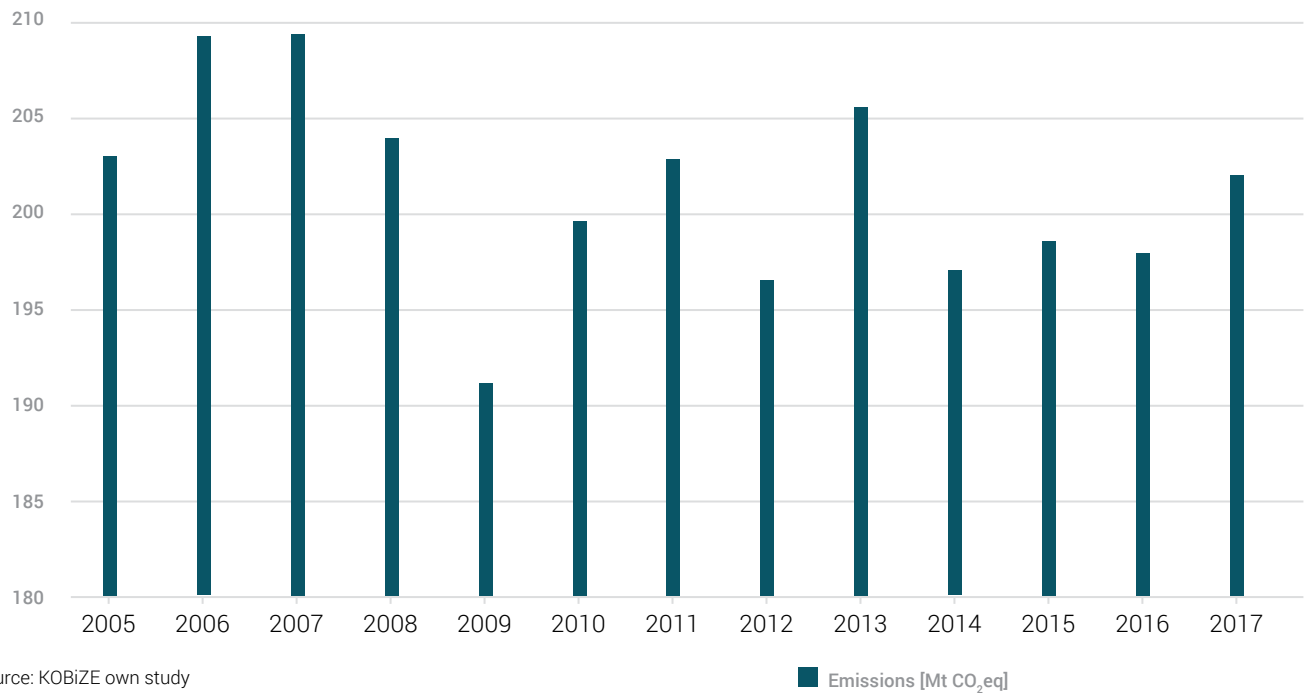
Fig. 35. Carbon dioxide emissions from installations covered by the EU ETS in the years 2005- 2017, expressed in Mt CO 2 eq
