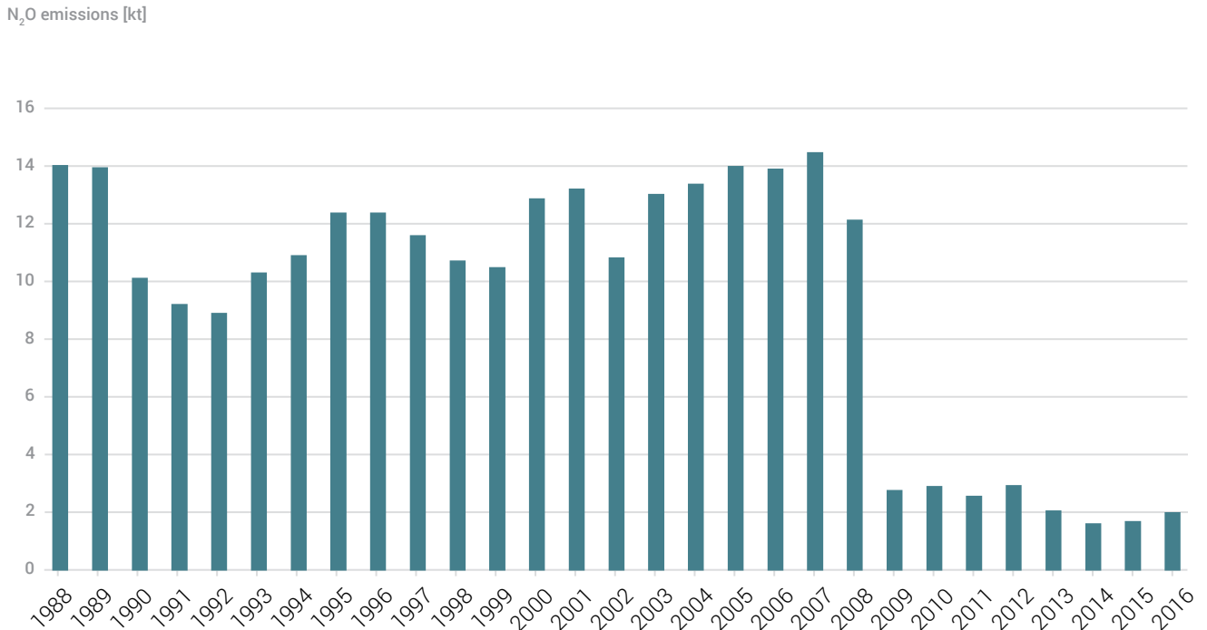
Fig. 20. Changes in the emission of nitrous oxide from nitric acid production in Poland, 1988-2016
